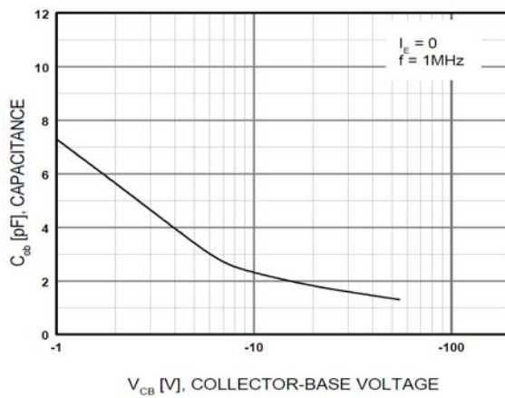
Figure 3. Output Capacitance
