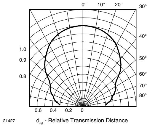
Fig. 10 - Horizontal Directivity
