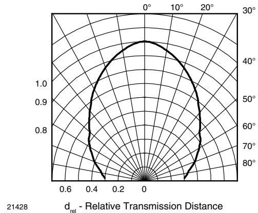
Fig. 11 - Vertical Directivity
