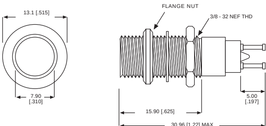
HOLDER WITHOUT COLLAR*
