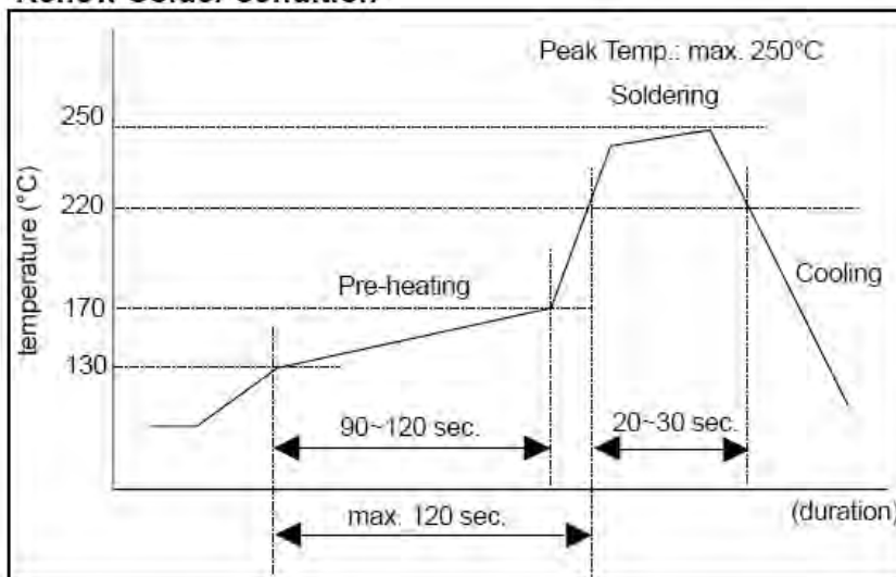
Reflow Solder condition
