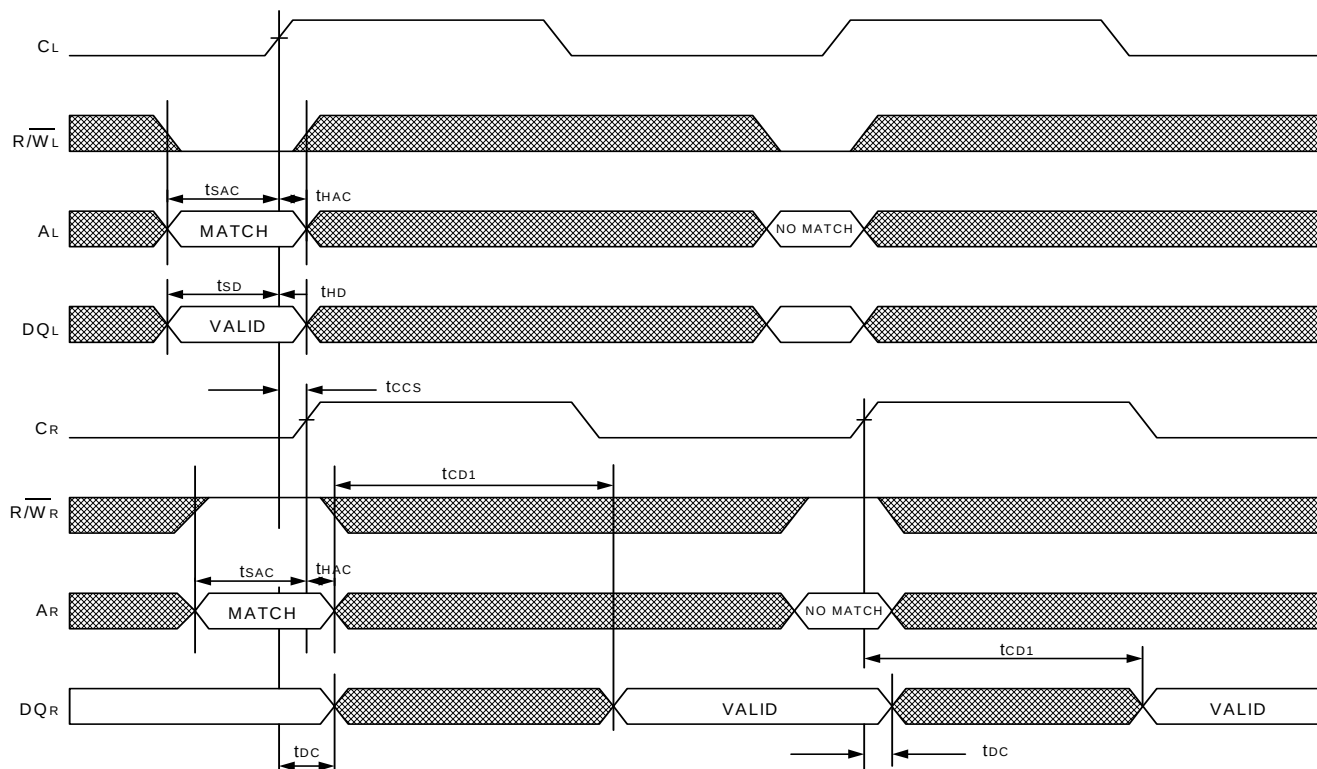
Figure 23. Port-to-Port WRITE-to-READ for Flow through Mode
