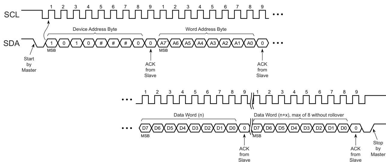
Figure 5-2. Page Write
