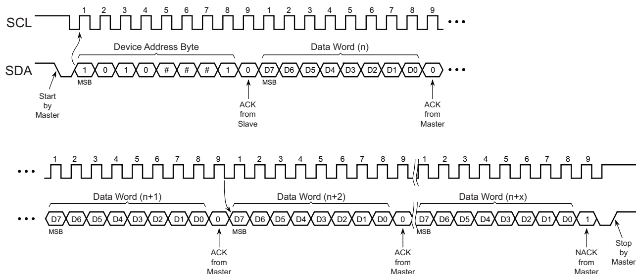
Figure 7-3. Sequential Read from a Current Address Read
