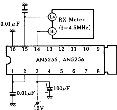
Test Circuit 2 ( R_i , C_i )
