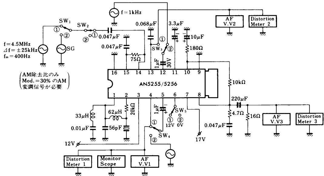
Test Circuit 3 ( V_{i(lim)} , AMR, V_o , THD (IF) , A_{1t} , A_{13-5} , THD (AF) , P_o , G_v , THD (out) )
