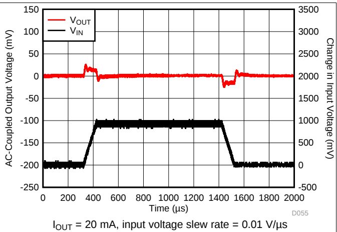
Figure 20. V_{IN} Transient
