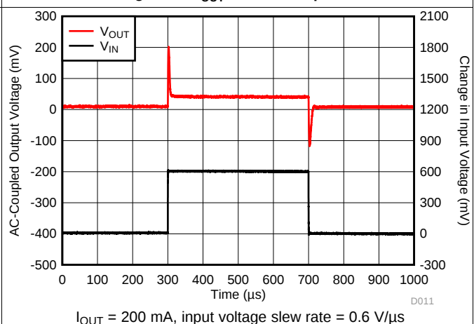
Figure 18. V_{IN} Transient
