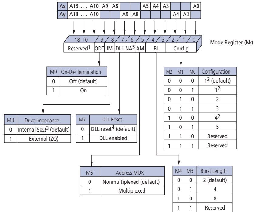
Figure 40: Mode Register Definition in Multiplexed Address Mode
