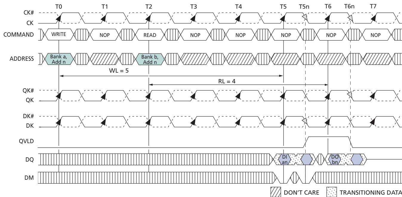
Figure 31: WRITE-to-READ
