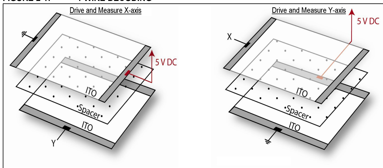
FIGURE 2-1: 4-WIRE DECODING
