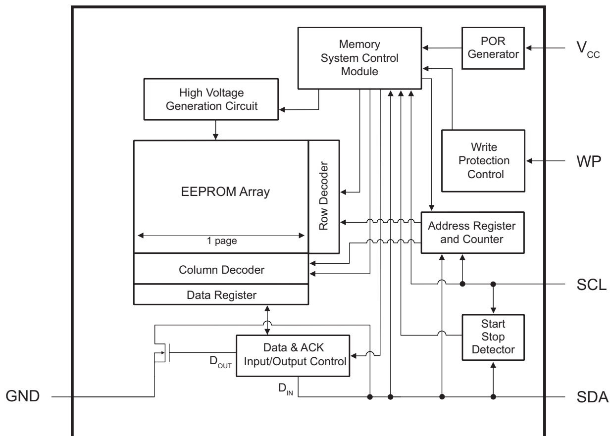
Figure 2-1. Block Diagram
