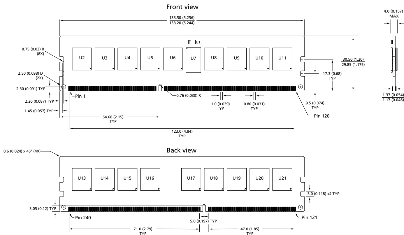
Figure 5: 240-Pin DDR3 RDIMM (PCB 1560)
