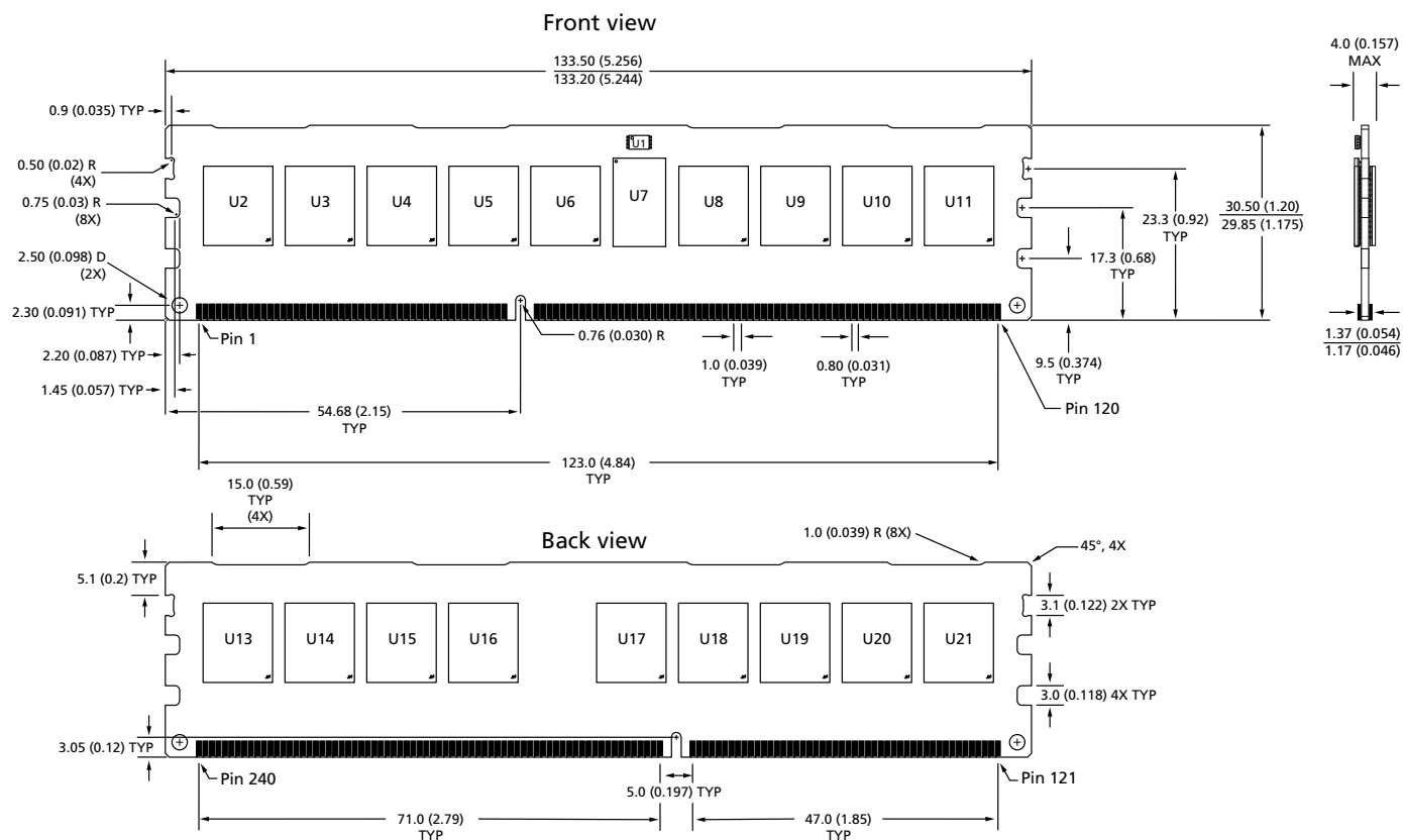
Figure 4: 240-Pin DDR3 RDIMM (PCB 1164)
