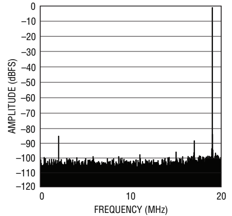
LTC2171-14: 8k Point FFT, f_{IN} = 139\text{MHz} , -1\text{dBFS} , 40\text{Mpsps}
