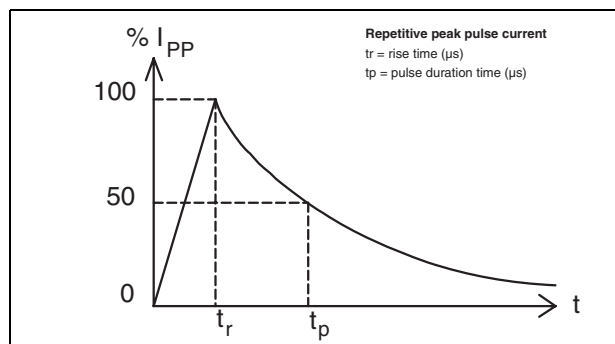
Figure 1. Pulse waveform (10/1000 \mu\text{s} )
