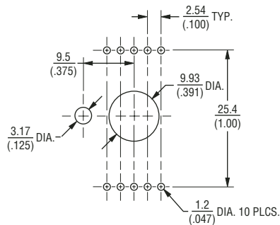
PCB Board Hole Pattern w/PCB Bracket
