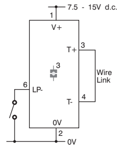
With internal (switched) backlight supply. Short link 3.
