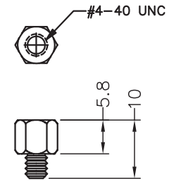
JACKSCREW DETAIL
