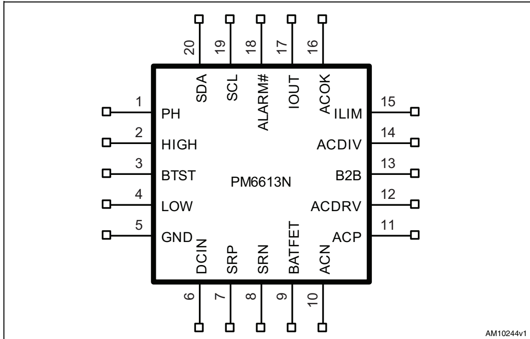
Figure 2. PM6613N pinout
