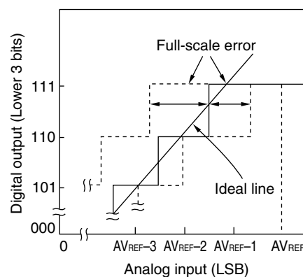
Figure 11-15. Full-Scale Error
