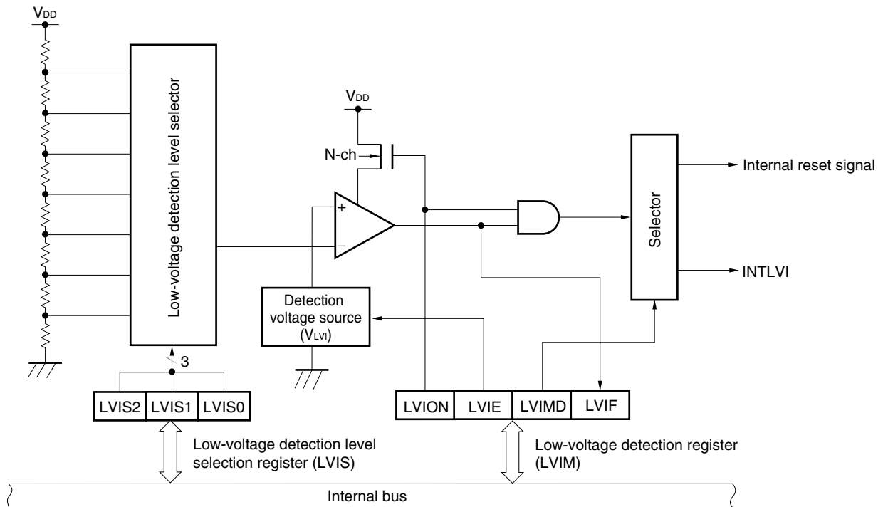
★ Figure 21-1. Block Diagram of Low-Voltage Detector
