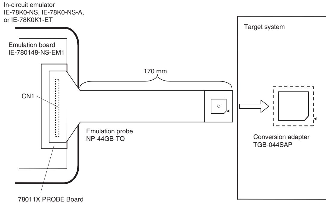
Figure B-1. Distance Between IE System and Conversion Adapter
