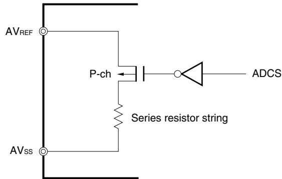
Figure 11-18. Circuit Configuration of Series Resistor String
