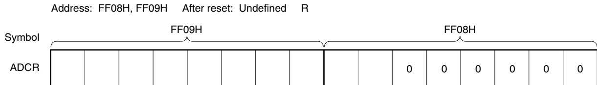
Figure 11-5. Format of A/D Conversion Result Register (ADCR)
