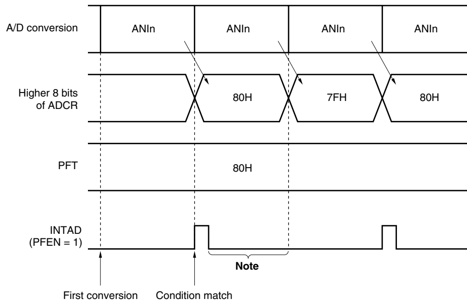
Figure 11-11. Power-Fail Detection (When PFEN = 1 and PFCM = 0)
