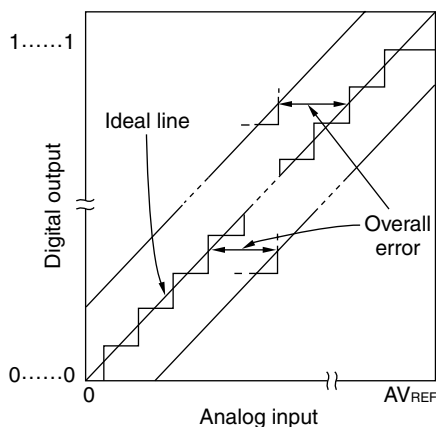
Figure 11-12. Overall Error
