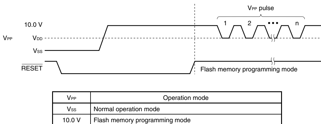
Figure 23-18. Flash Memory Programming Mode
