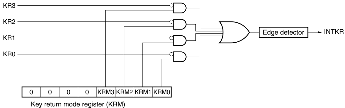
Figure 16-1. Block Diagram of Key Interrupt
