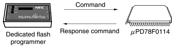
Figure 23-19. Communication Commands
