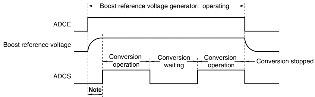
Figure 11-3. Timing Chart When Boost Reference Voltage Generator Is Used
