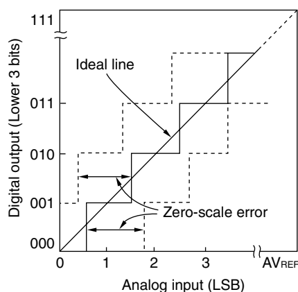
Figure 11-14. Zero-Scale Error
