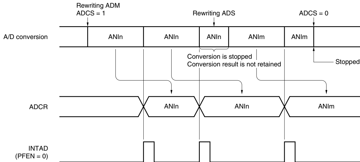
Figure 11-10. A/D Conversion Operation
