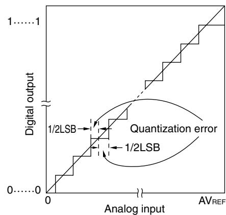
Figure 11-13. Quantization Error
