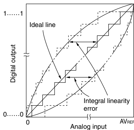
Figure 11-16. Integral Linearity Error
