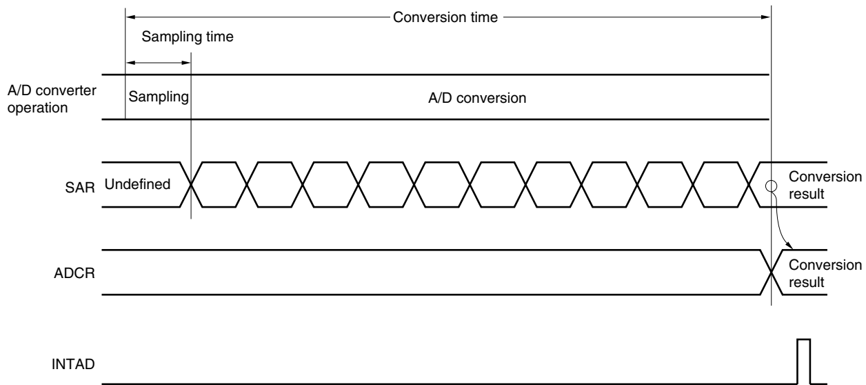
Figure 11-8. Basic Operation of A/D Converter
