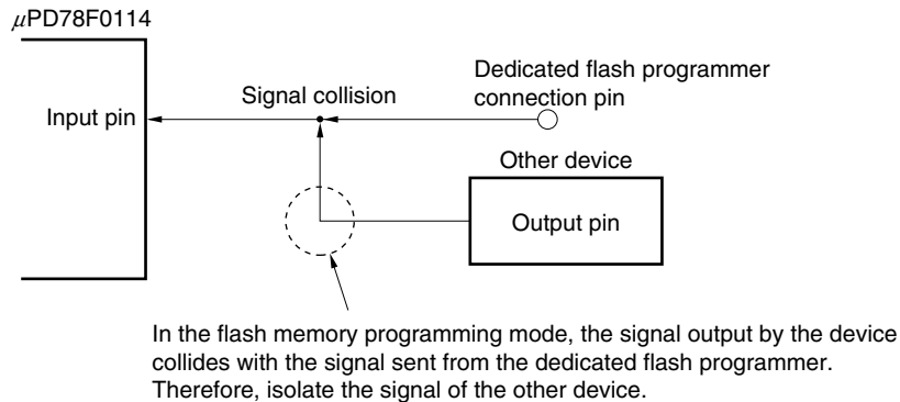
Figure 23-14. Signal Collision (Input Pin of Serial Interface)
