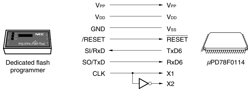
Figure 23-12. Communication with Dedicated Flash Programmer (UART6)
