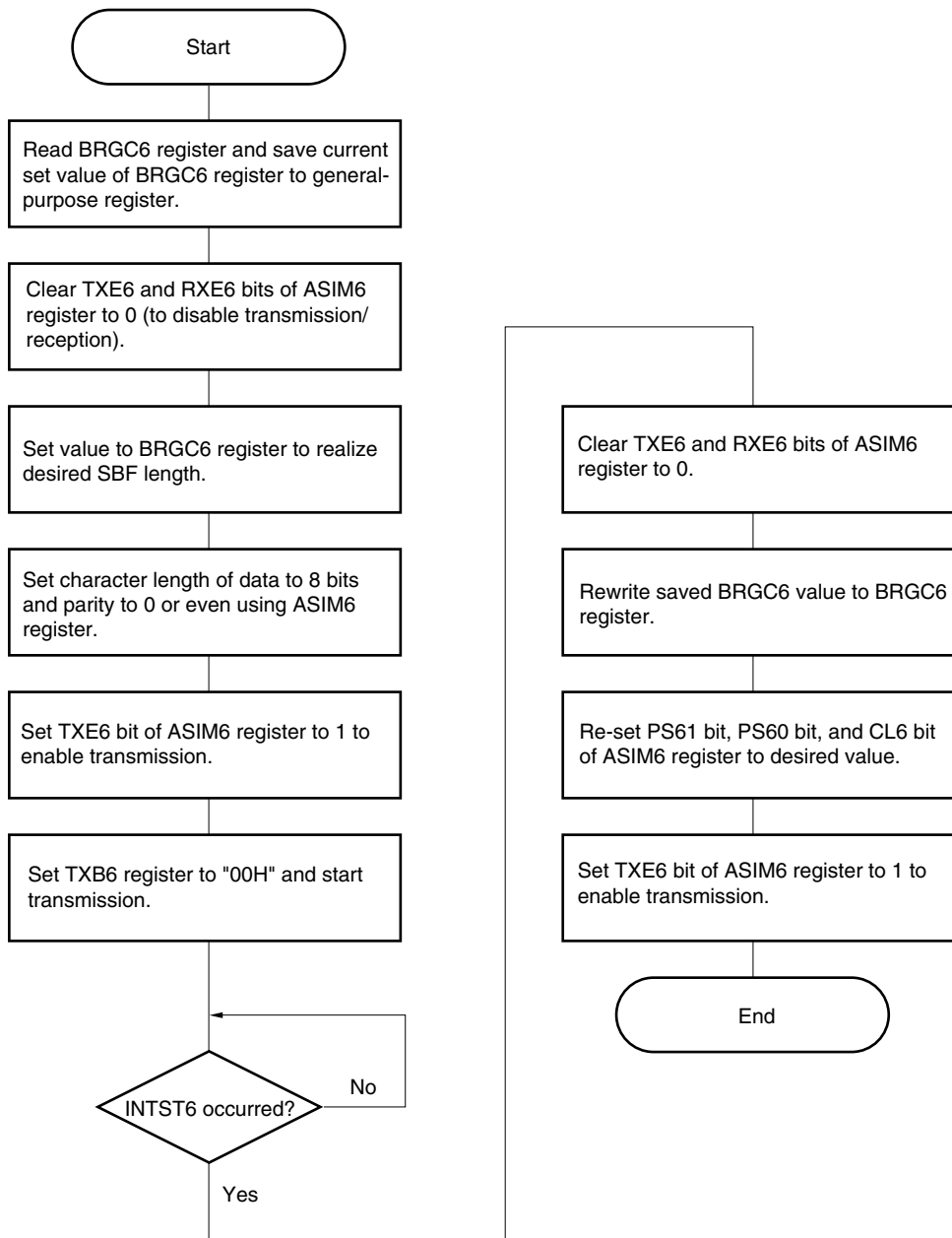
Figure 13-23. SBF Transmission
