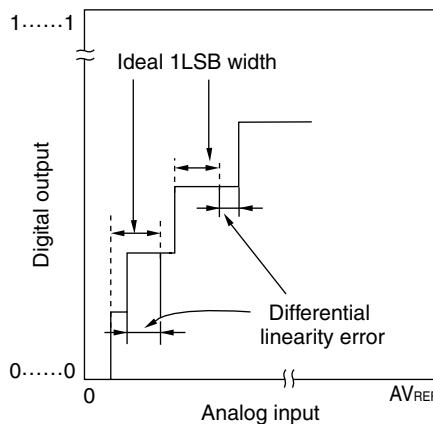
Figure 11-17. Differential Linearity Error
