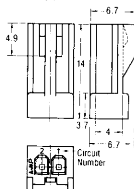
2 Position Housing
