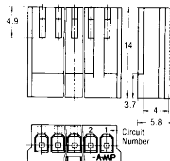
3 ~ 12 Position Housing
