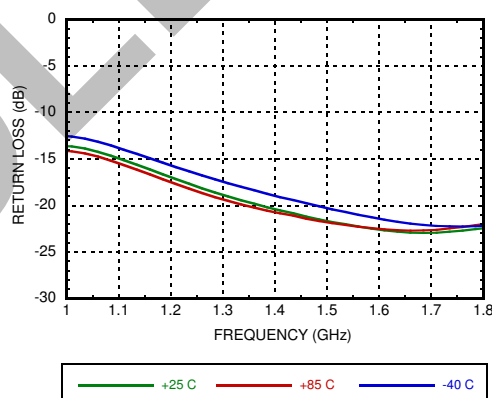
Input Return Loss vs. Temperature [2]
