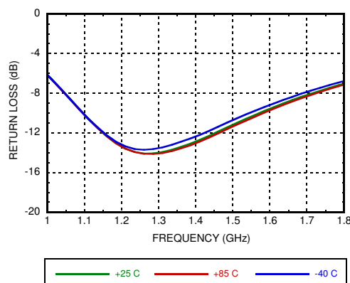
Output Return Loss vs. Temperature [2]
