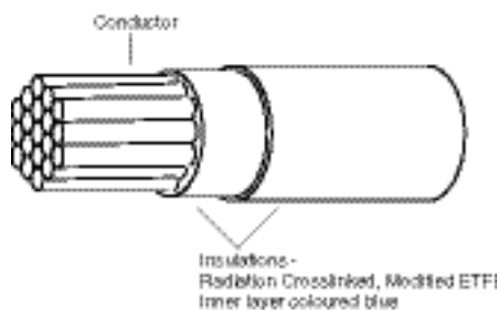
SPEC 55 insulation system - dual wall
