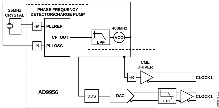
Figure 22. Dual-Clock Configuration
