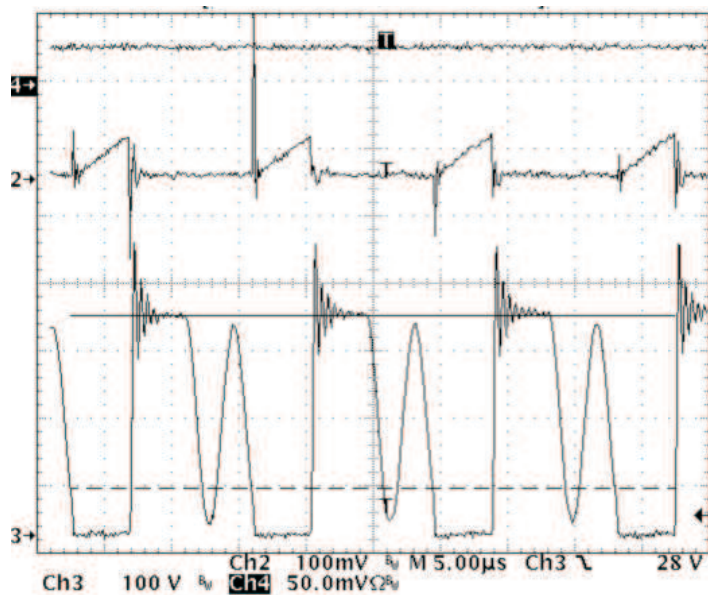
Figure 20. Current Sense Waveform (Ch2 - R11 current sense, Ch3 - switch node voltage and Ch4 - LED current)
