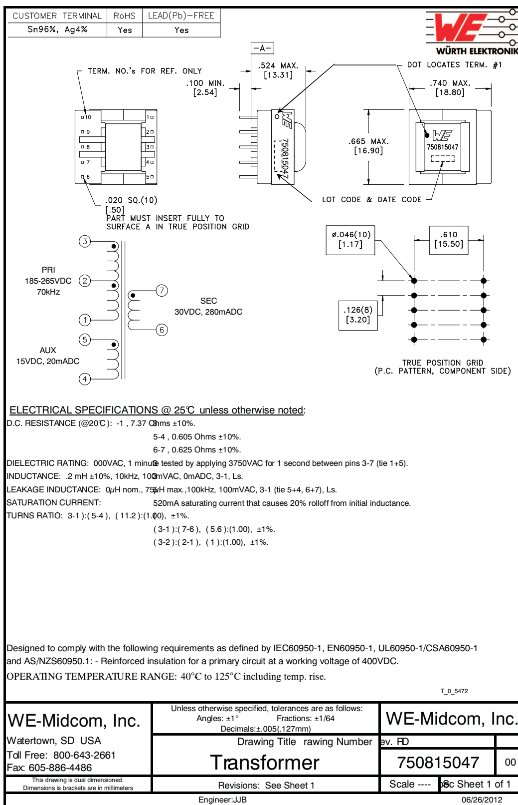
Figure 28. Transformer Specification
