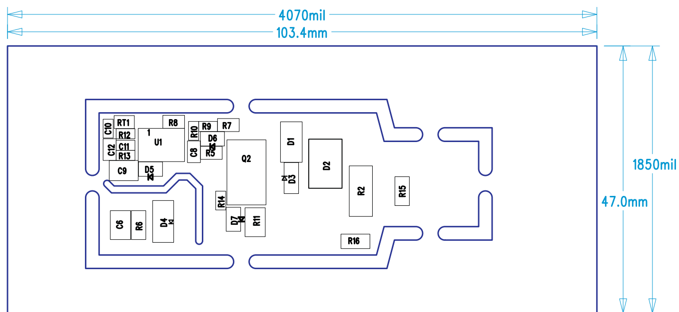
Figure 32. LM3447-A19-230VEVM Bottom Assembly Drawing (bottom view)
