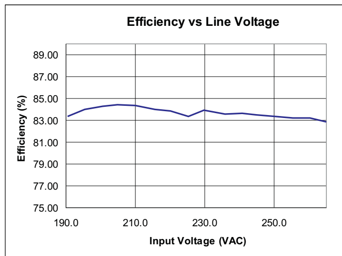
Figure 3. LM3447-A19-230VEVM Efficiency
