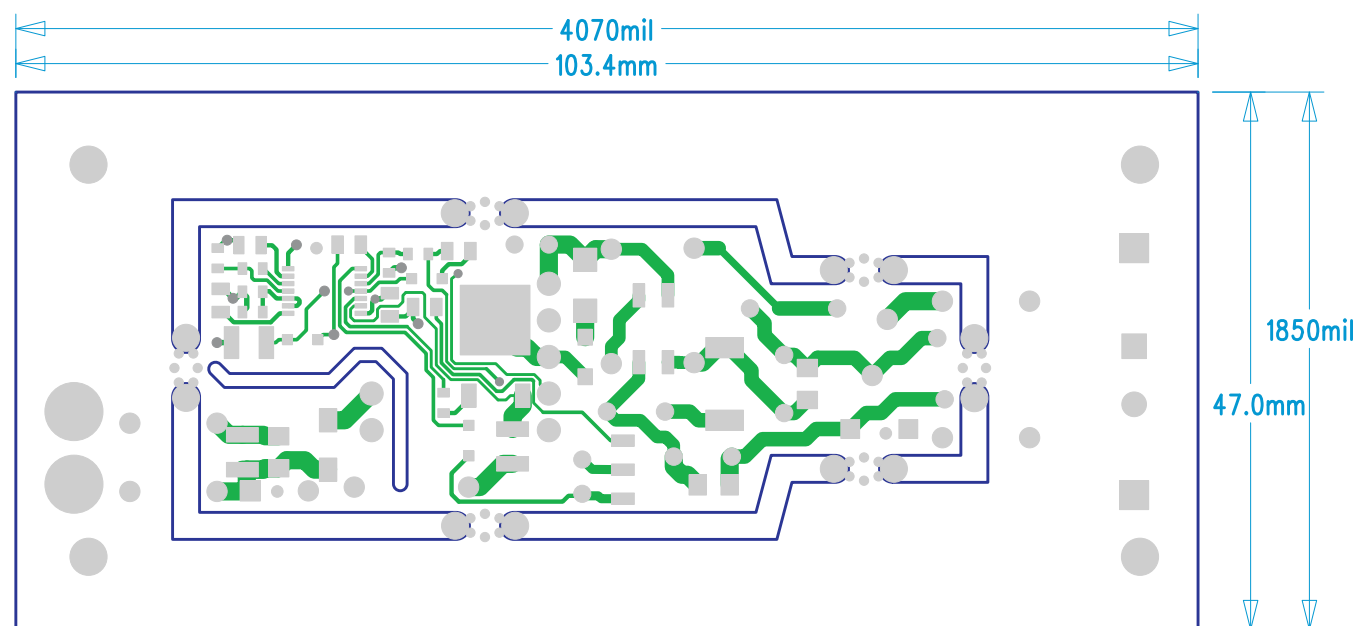
Figure 30. LM3447-A19-230VEVM Bottom Layer Copper (bottom view)
