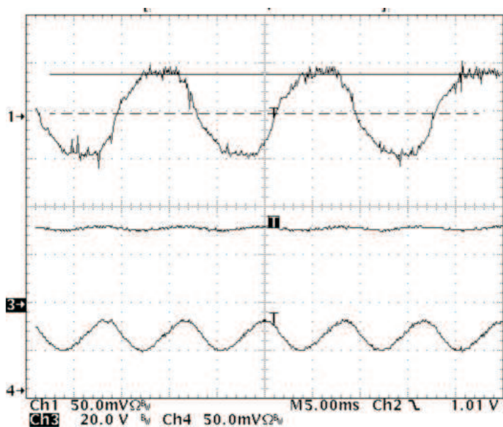
Figure 21. Pre-Open Circuit Waveforms (Ch1 - line current, Ch3 - LED voltage and Ch4 - LED current)
