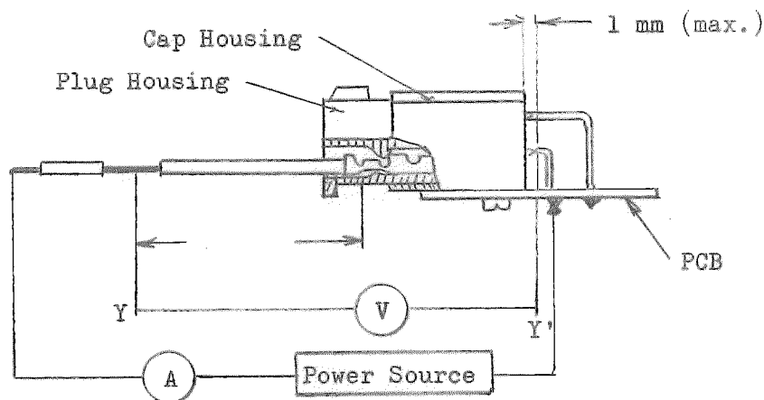
Fig. 1 - B Resistance Testing Circuit for Horizontal Housing
