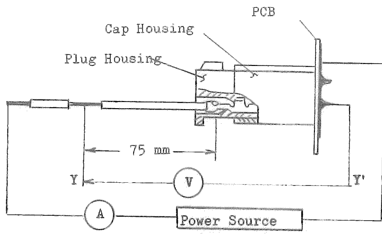
Fig. 1 - A Resistance Testing Circuit for Vertical Housing
