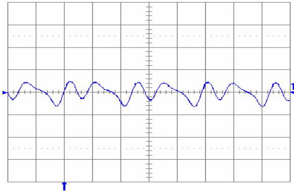
Fig. 1.0V.13: Output voltage ripple (20 mV/div.) at full rated load current into a resistive load with C_o = 10 μF tantalum + 1 μF ceramic and V_{in} = 48 V. Time scale: 1 μs/div.
