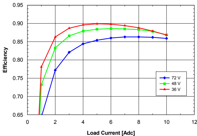
Fig. 5.0V.5: Efficiency vs. load current and input voltage for SQ48T/S10050 converter mounted vertically with air flowing from pin 3 to pin 1 at a rate of 300 LFM (1.5 m/s) and T_a = 25 °C.
