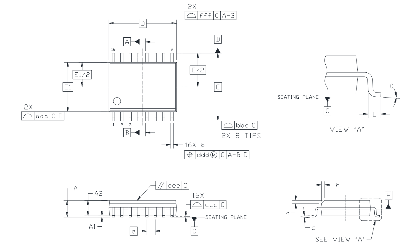
Figure 17. 16-Pin Wide Body SOIC
