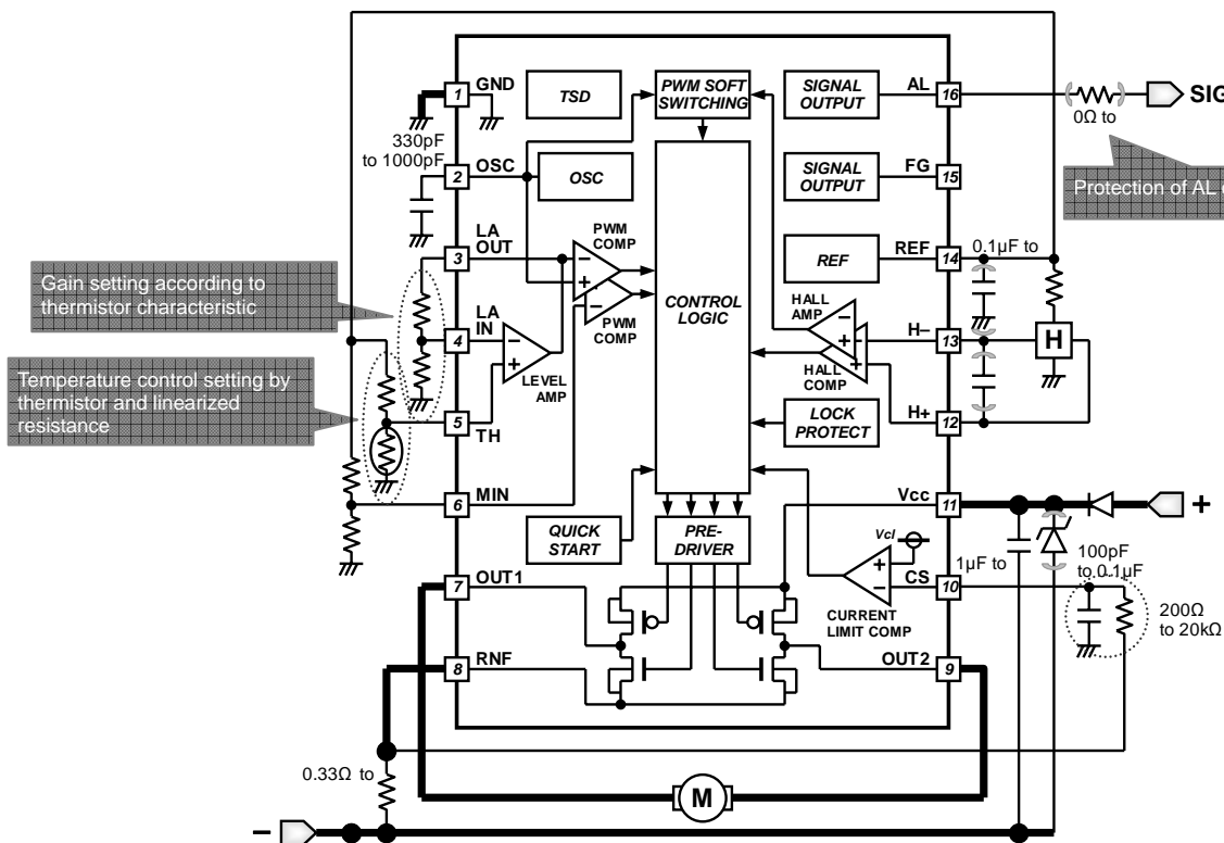
Fig.26 Thermistor controllable 3 wires type (AL) motor application circuit
