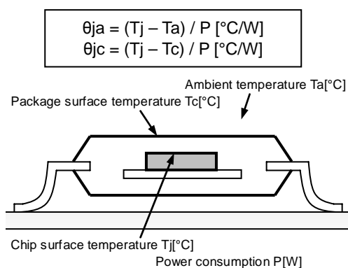
Fig.27 Thermal resistance
