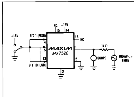
Figure 7. Output Capacitance
