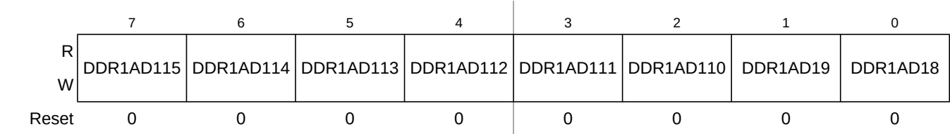
Figure 22-71. Port AD1 Data Direction Register 1 (DDR1AD1)
