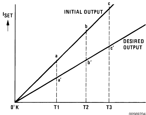
FIGURE 2. Gain Adjustment
