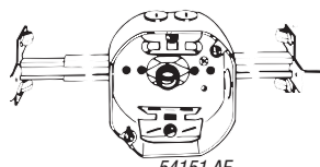
54151 AF Octagon box mounted on adjustable bar hanger 50 lb. load max rating
