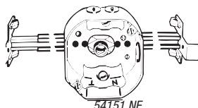
54151 NF Octagon box mounted on adjustable bar hanger. 50 lb. load max rating
