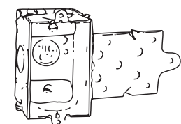
806-SW-1/4 "S" bracket recessed 1/4"
