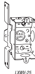
LXWV-25 "CV" bracket recessed 1/8"
