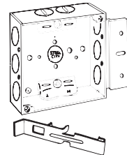
52151 MS N* "MS" bracket for 1½", 2½", 3½", 4"
