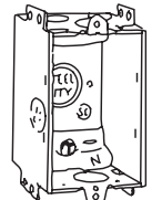
A-258 Without nails
