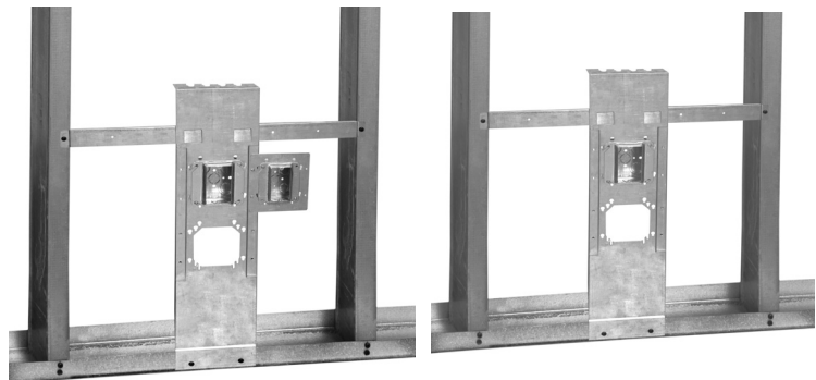
SV1218 mounted to floor track and studs with one 4" square box installed and optional SVX adapter plate with one box installed.
