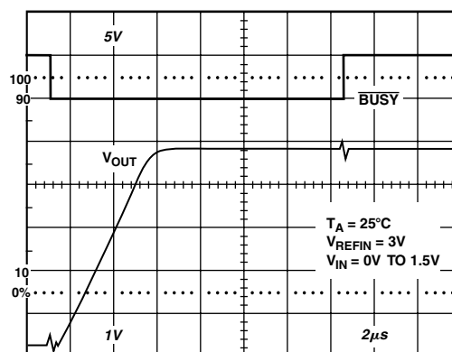
TPC 4. Acquisition Time and Output Settling Time
