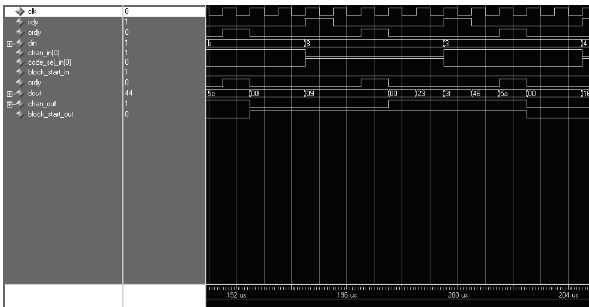
Figure 4. User Interface Timing Diagram for Two-channel Correlator
