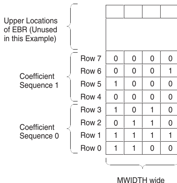
Figure 7. Example Coefficient Sequences Written in Coefficient Memory
