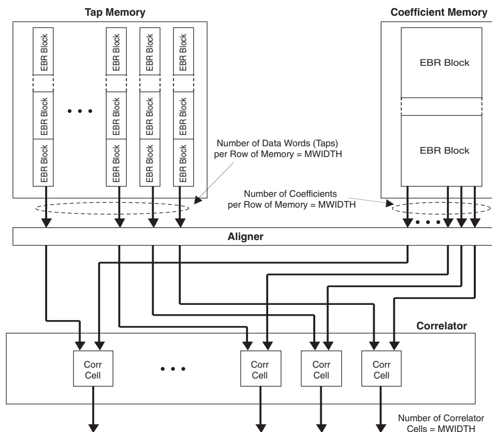
Figure 5. Tap and Coefficient Memories
