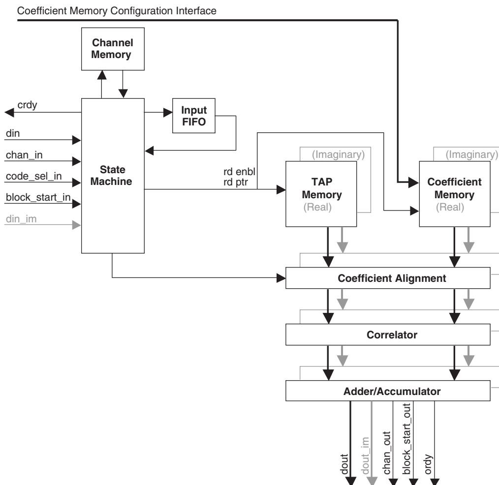
Figure 2. Correlator IP Core Block Diagram
