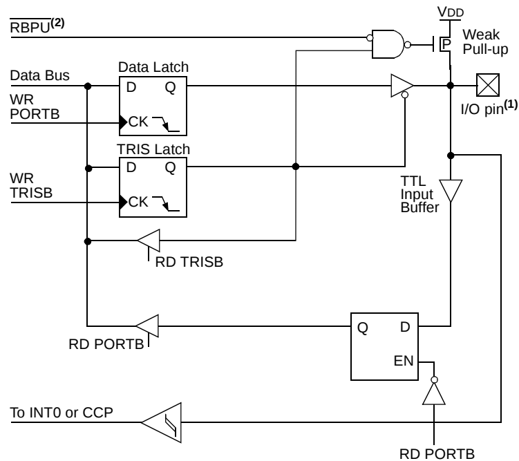
FIGURE 5-8: BLOCK DIAGRAM OF RB0 PIN
