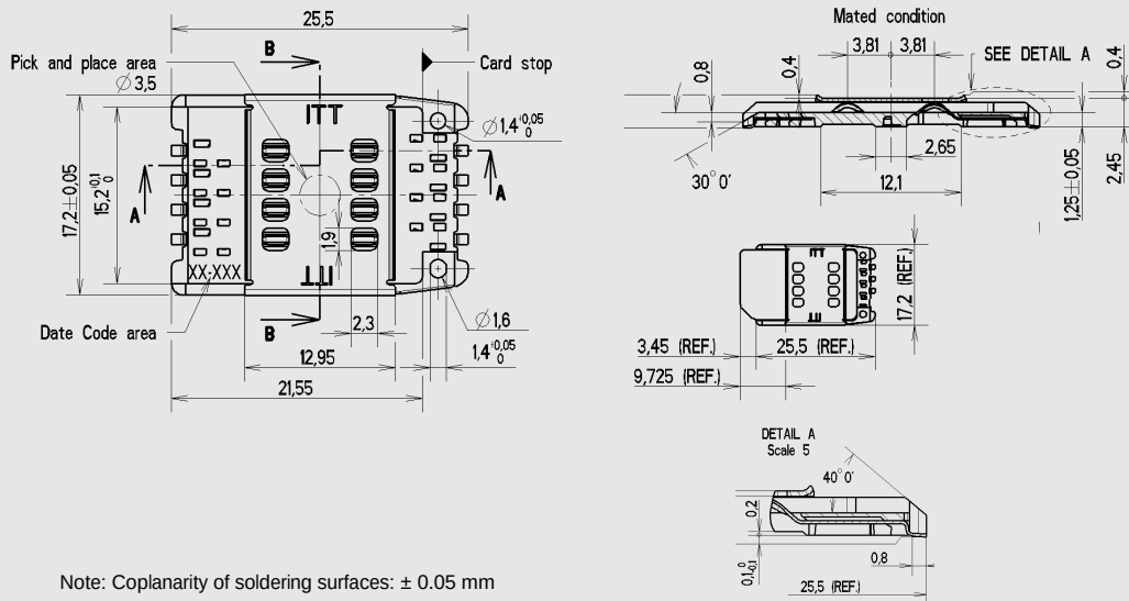
Fixed cover CCM03-3505 (6 contacts not shown) / CCM03-3504 (8 contacts)
