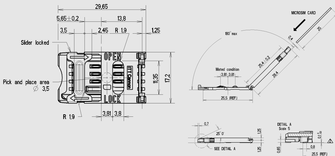
Hinged Cover CCM03-3013 (6 contacts + Card Detect Switch)
