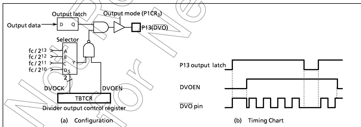
Figure 2-9. Divider Output
