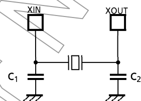
(1) High-frequency Oscillation
