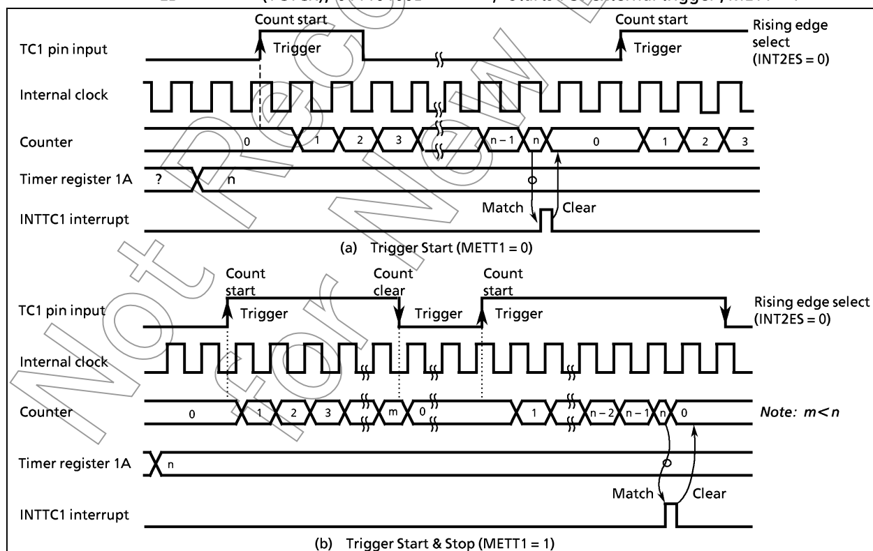
Figure 2-13. External Trigger Timer Mode Timing Chart
