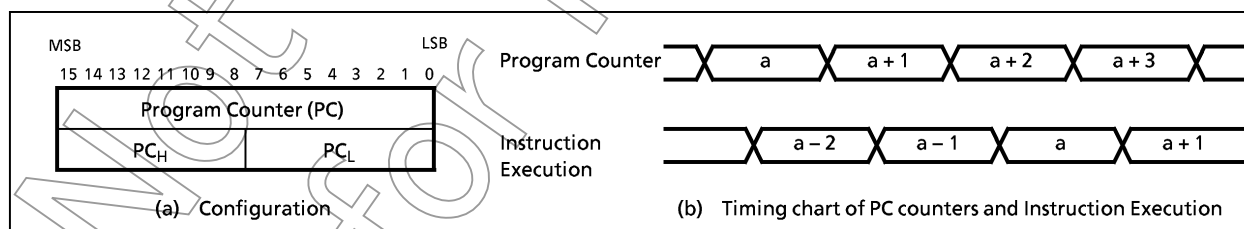
Figure 1-3. Program Counter
