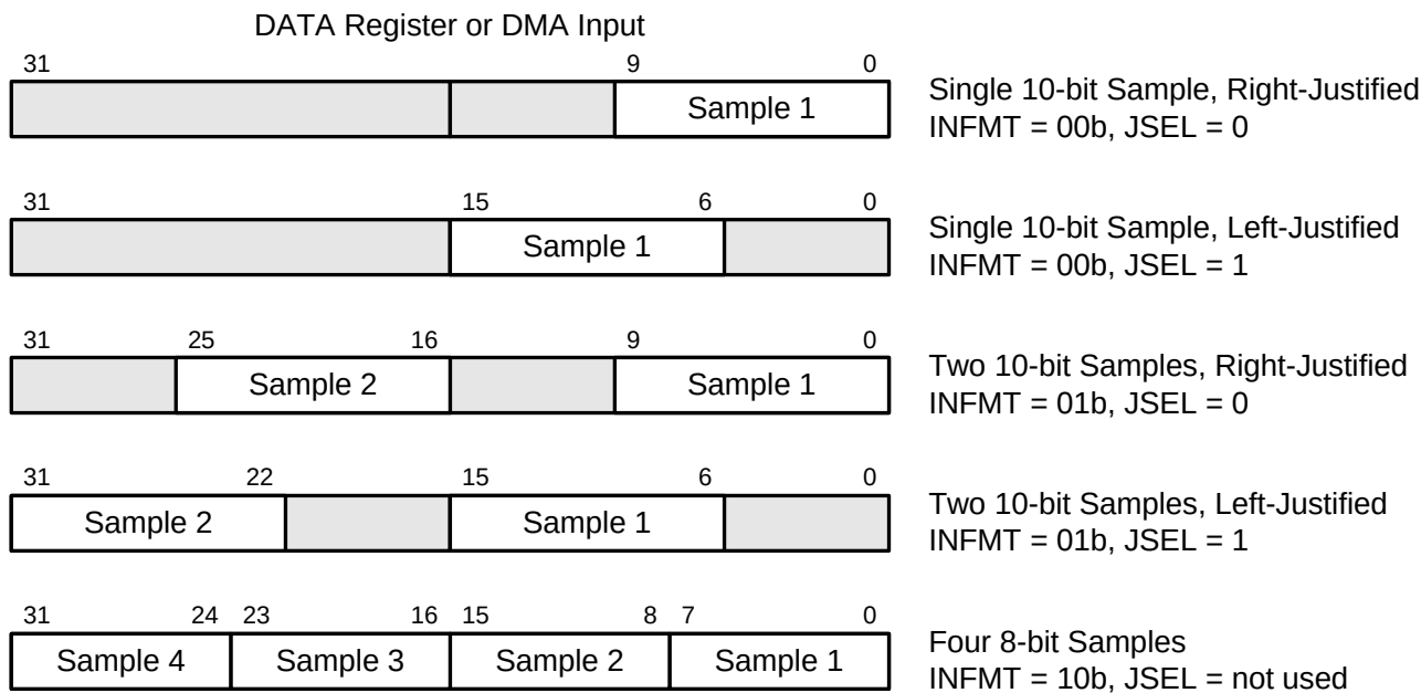
Figure 24.2. Data Packing Modes and Data Justification
