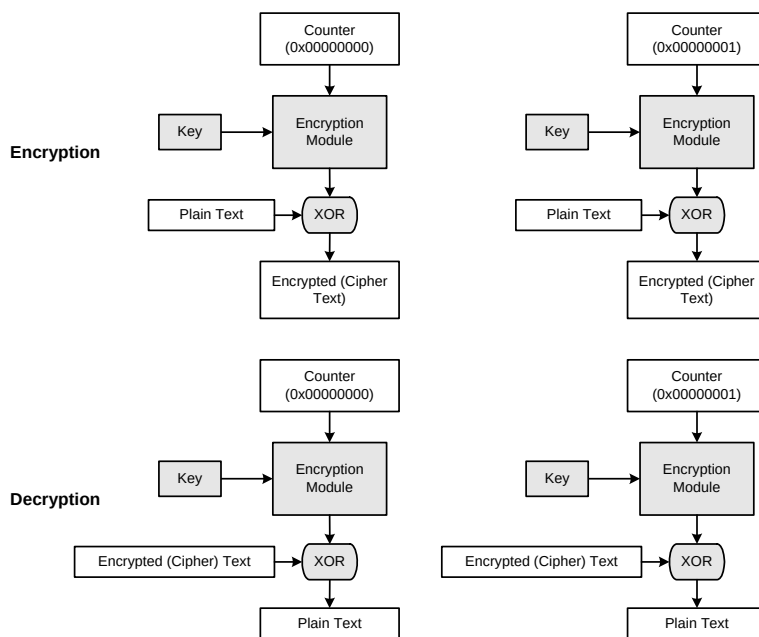
Figure 12.11. Counter (CTR) Algorithm Diagram
