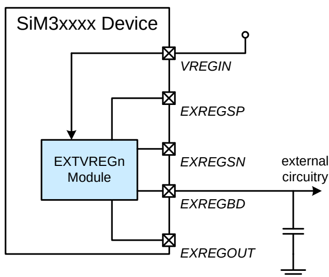
Figure 20.4. External Regulator in Standalone Mode
