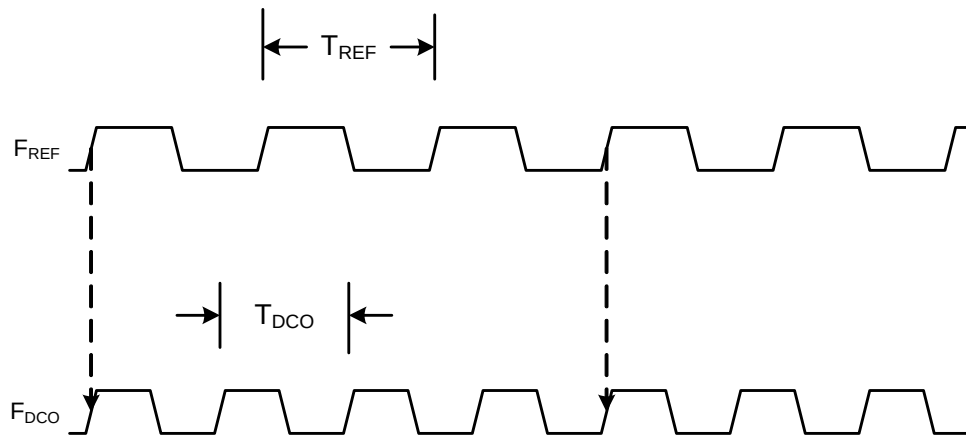
Figure 30.4. Phase-Lock Mode
