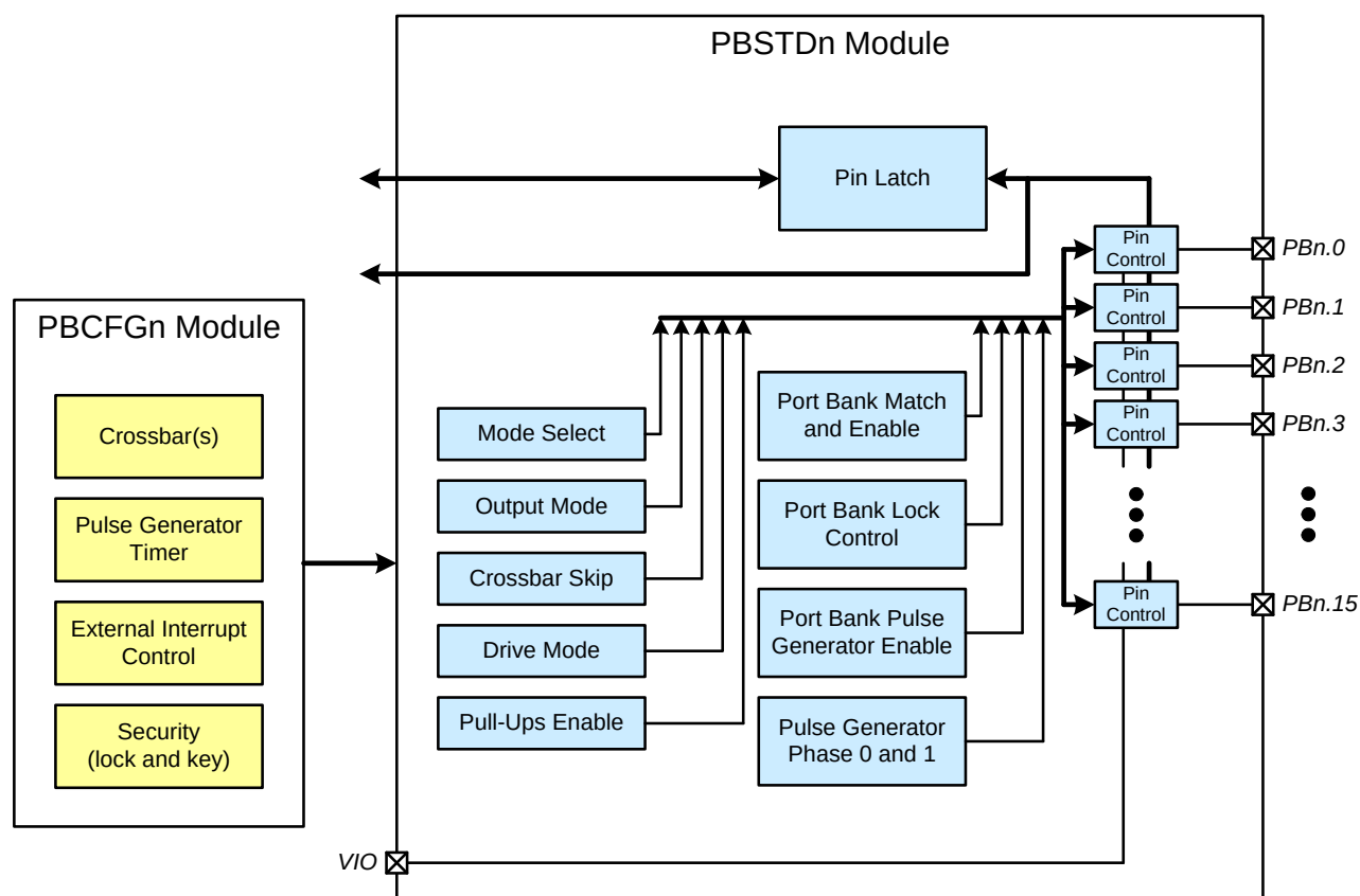
Figure 8.5. PBSTD Block Diagram
