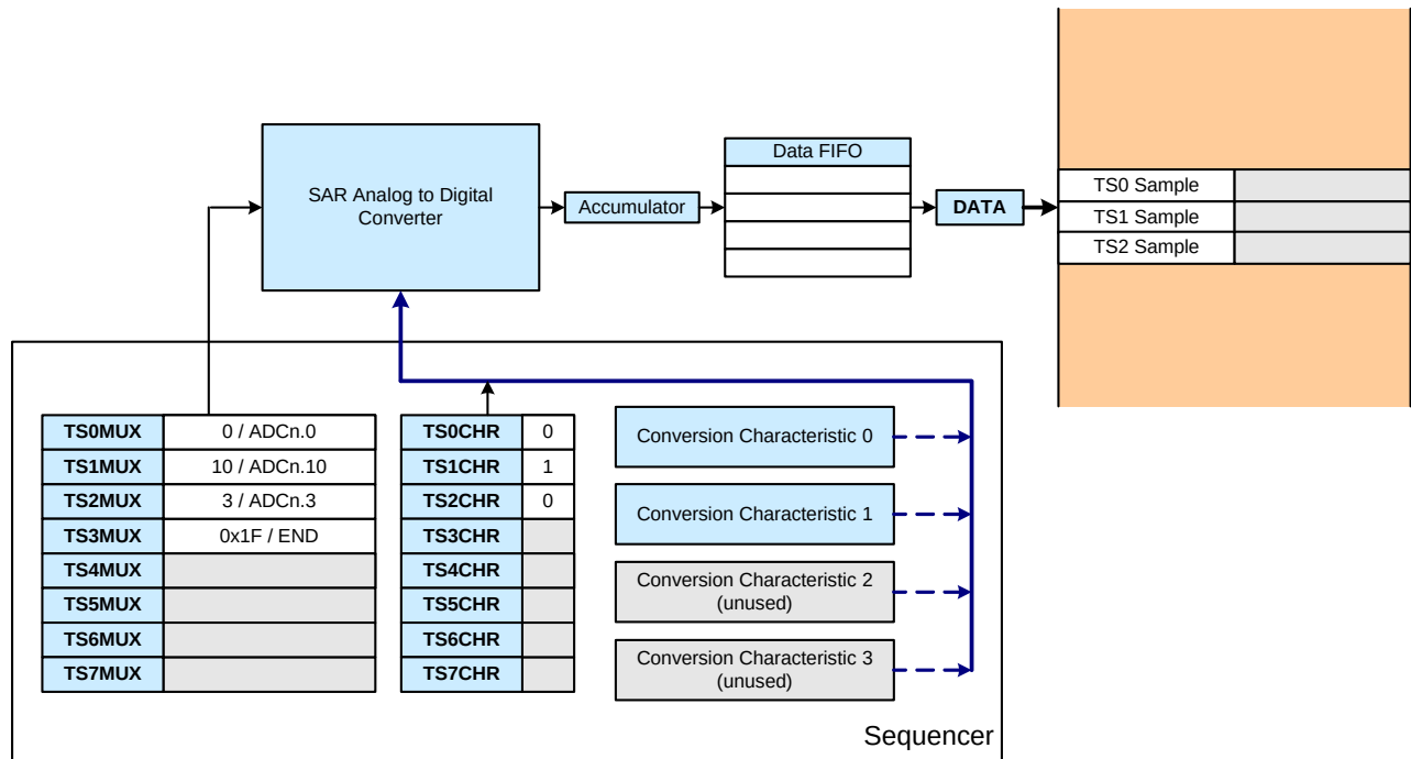
Figure 32.6. Channel Scan Setup and Timing
