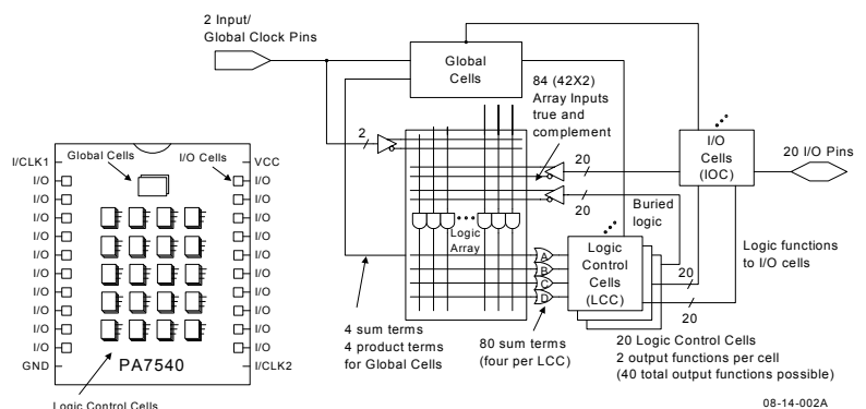
Figure 2. Block Diagram
