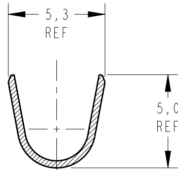
SECTION C-C SCALE 5:1
