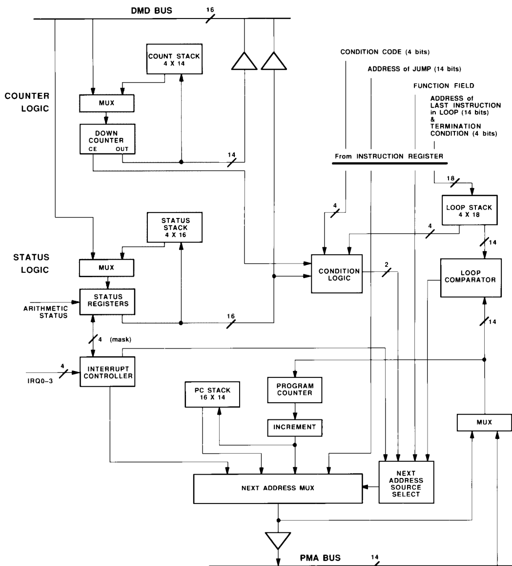
Figure 6. Program Sequencer
