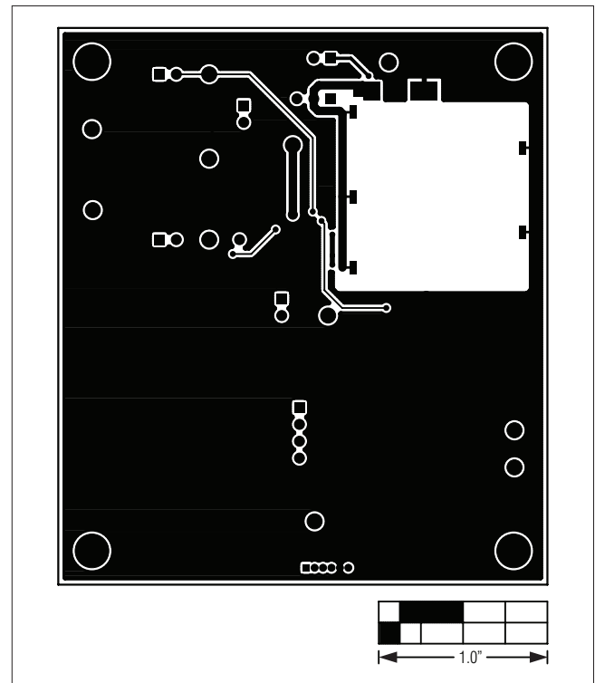
Figure 5. MAX17710 EV Kit PCB Layout—Solder Side
