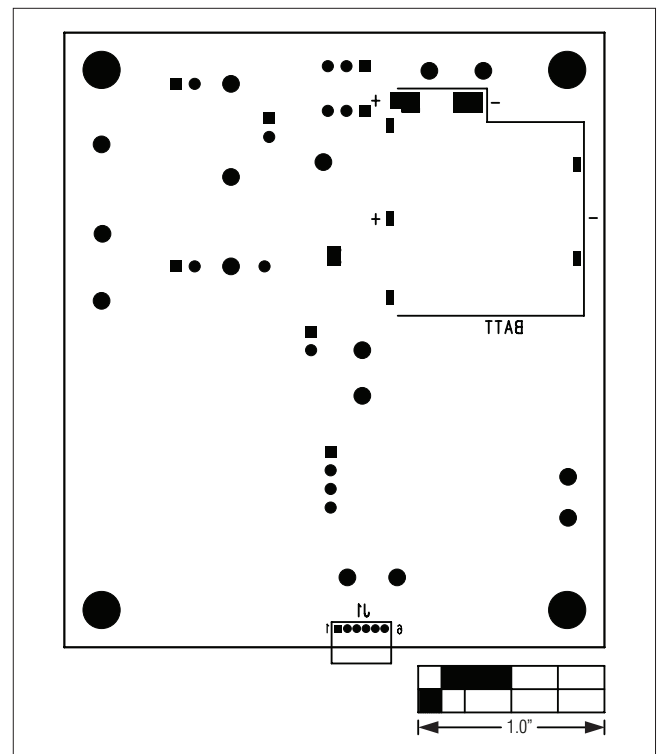
Figure 6. MAX17710 EV Kit Component Placement Guide—Solder Side
