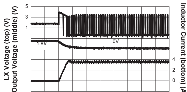
Step-Down Converter Short Circuit Protection ( V_{IN} = 5V ; V_{OUT} = 1.8V ; C_{FF} = 100pF )
