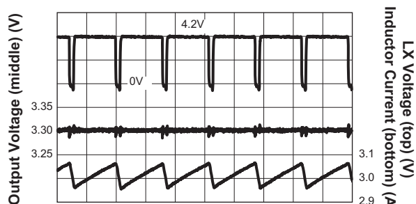
Step-Down Converter Output Ripple ( V_{IN} = 4.2V ; V_{OUT} = 3.3V ; I_{OUT} = 3A )
