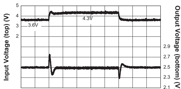
Step-Down Converter Line Transient Response ( V_{IN} = 3.6V to 4.3V ; V_{OUT} = 2.5V ; I_{OUT} = 3A )
