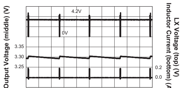
Step-Down Converter Output Ripple ( V_{IN} = 4.2V ; V_{OUT} = 3.3V ; I_{OUT} = 1mA )
