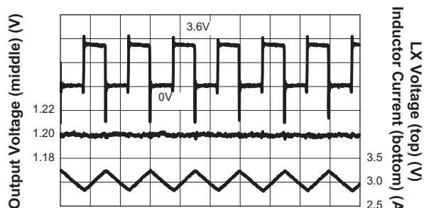
Step-Down Converter Output Ripple ( V_{IN} = 3.6V ; V_{OUT} = 1.2V ; I_{OUT} = 3A )
