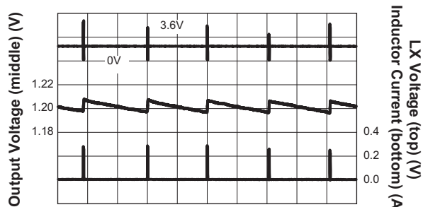
Step-Down Converter Output Ripple ( V_{IN} = 3.6V ; V_{OUT} = 1.2V ; I_{OUT} = 1mA )
