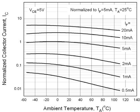
Figure 3. Normalized Collector Current vs Ambient Temperature
