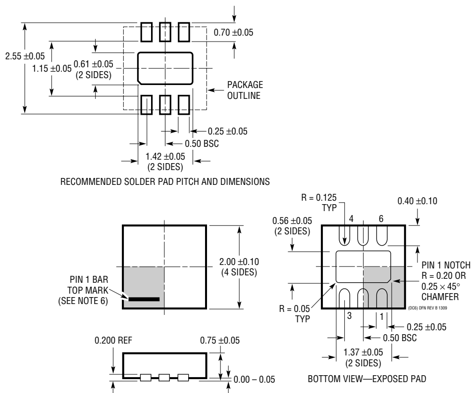
DC6 Package 6-Lead Plastic DFN (2mm × 2mm) (Reference LTC DWG # 05-08-1703 Rev B)
