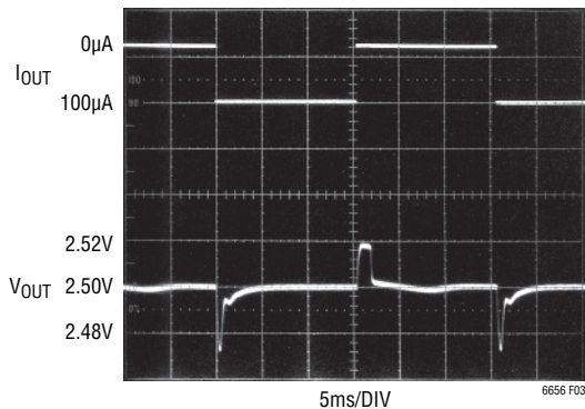
Figure 3. Transient Response, 0μA to 100μA Load Step (R2 = 24.9k, R1 = Open)
