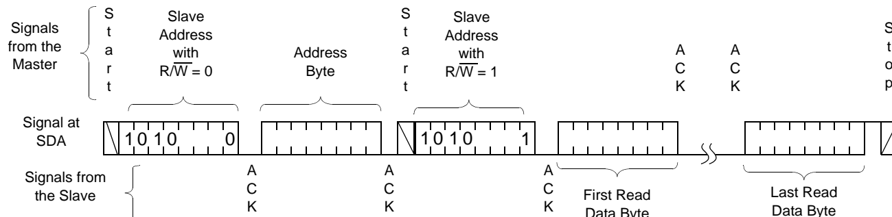
Figure 18. Read Sequence
