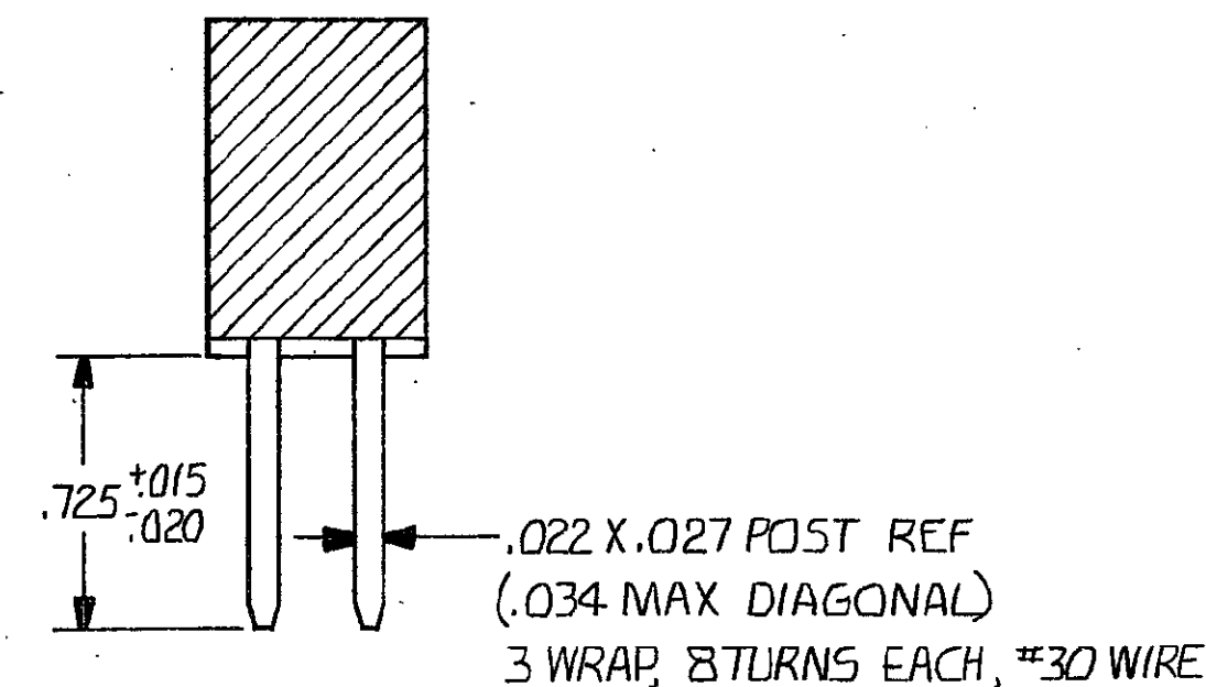
SECTION A-A WRAP TYPE CONTACT, PC MOUNT (TYPE V)
