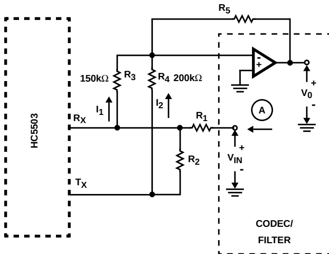
FIGURE 6. TRANSHYBRID CIRCUIT
