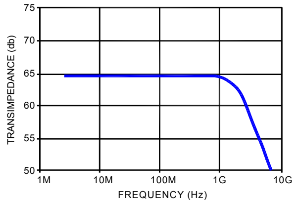
Fig. 6: TOTAL FREQUENCY RESPONSE
