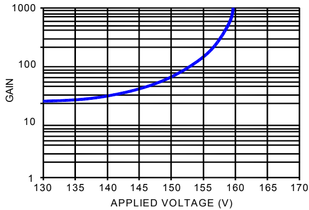
Fig. 1: APD GAIN vs BIAS VOLTAGE
