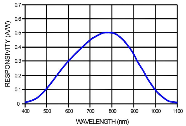
Fig. 2: APD SPECTRAL RESPONSE (M = 1)
