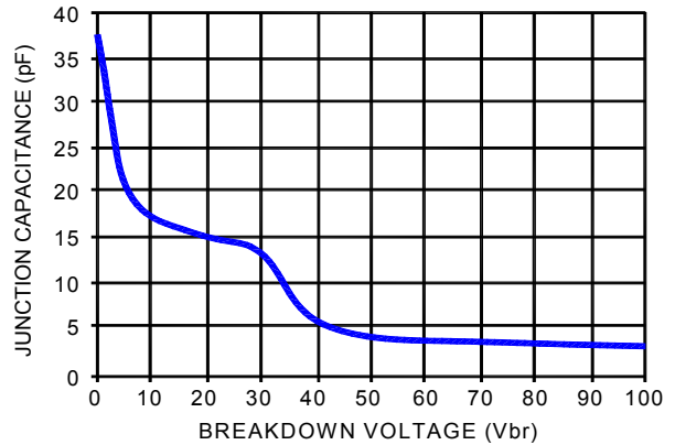
Fig.4 : APD CAPACITANCE vs VOLTAGE
