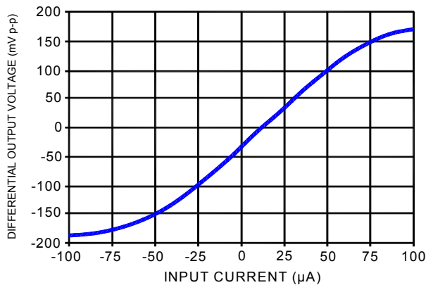
Fig. 5: AMPLIFIER TRANSFER FUNCTION
