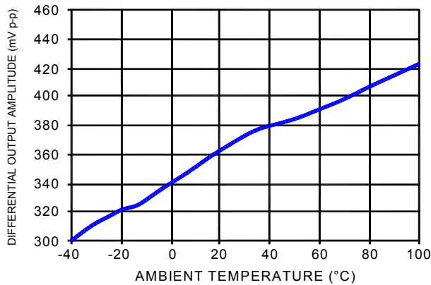
Fig. 3 : AMPLIFIER OUTPUT vs TEMPERATURE
