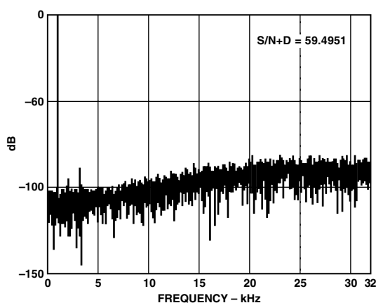
Figure 14. FFT (ADC 64 kHz Sampling)
